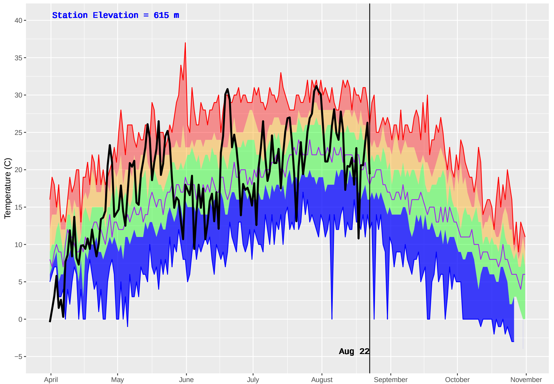
HIXON (187) : Historical (1976–2016) and Current (2018) Daily Temperature
